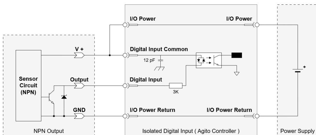
Figure 29. Digital Input with NPN Sensor
