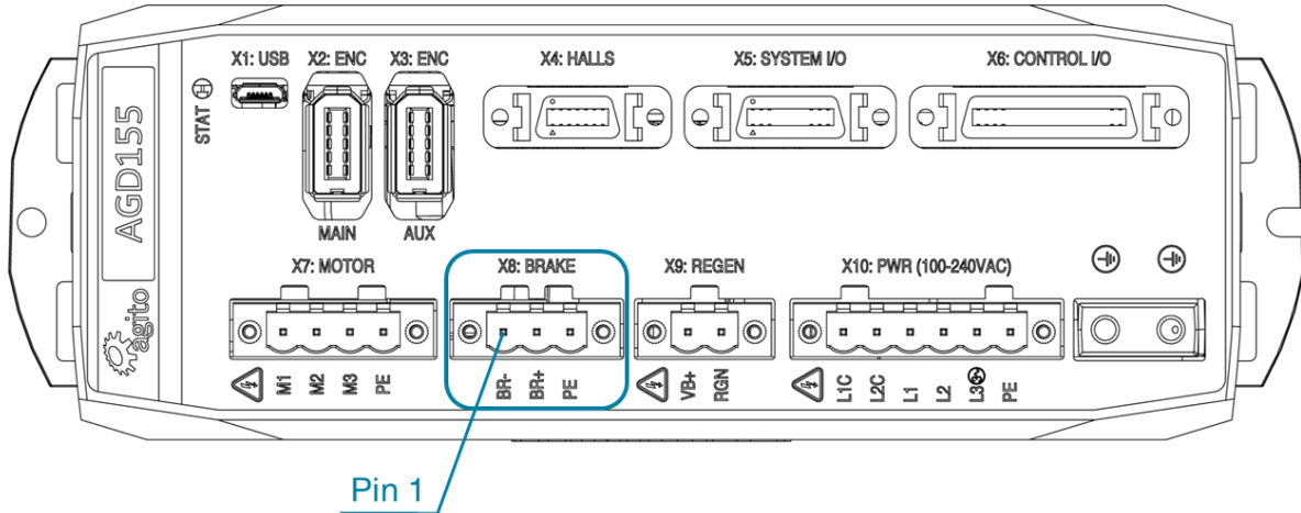
Figure 15. Brake Connector
