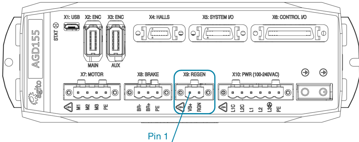
Figure 17. Regeneration Connector
