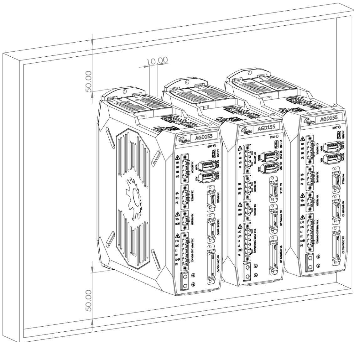
Figure 5. Mounting Multiple Units within Cabinet
