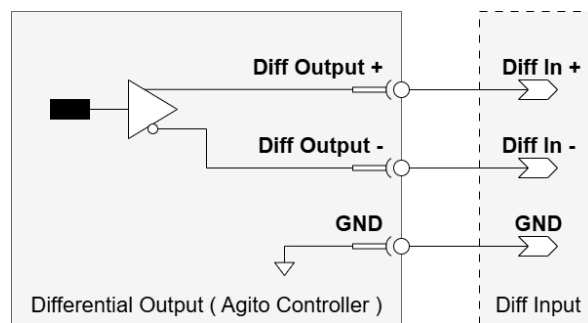
Figure 35. Differential Output
