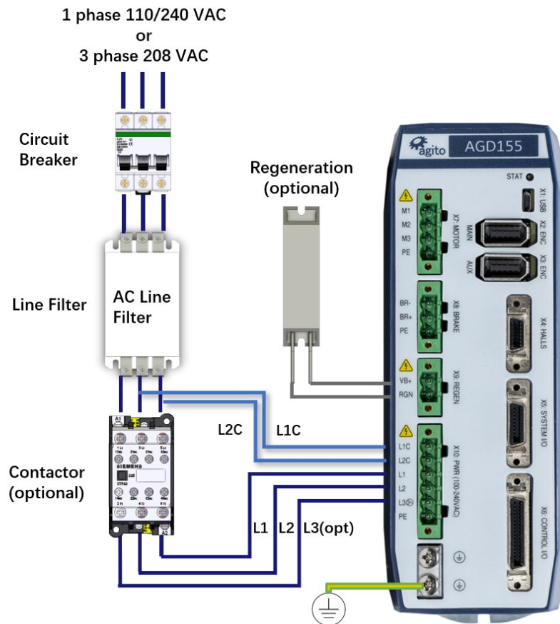
Figure 6. Power Supply Wiring
