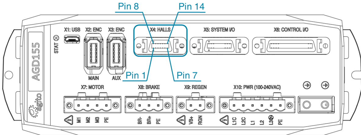
Figure 25. Hall Sensor Connector
