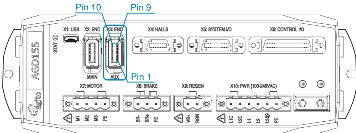
Figure 24. Aux Encoder Connector
