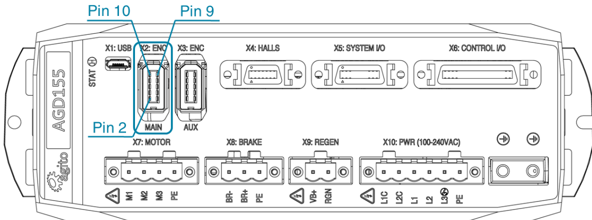
Figure 23. Main Encoder Connector
