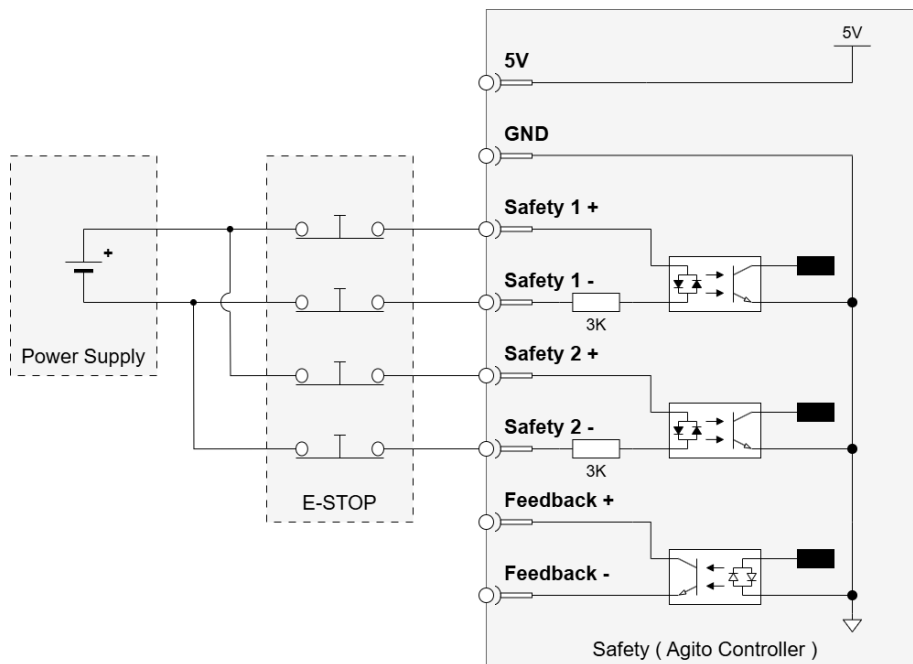
Figure 14. Safety with E-STOP
