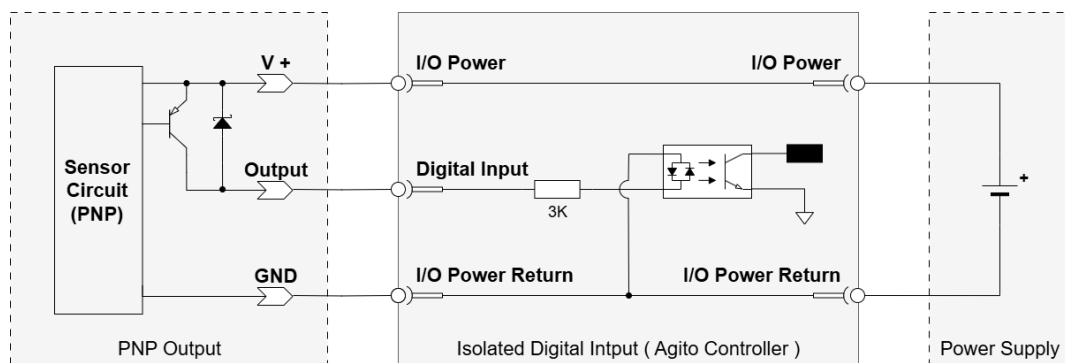
Figure 31. Digital Input 4
