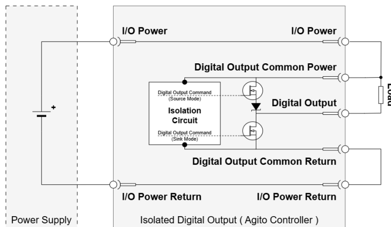
Figure 32. Digital Output (Sink Mode)
