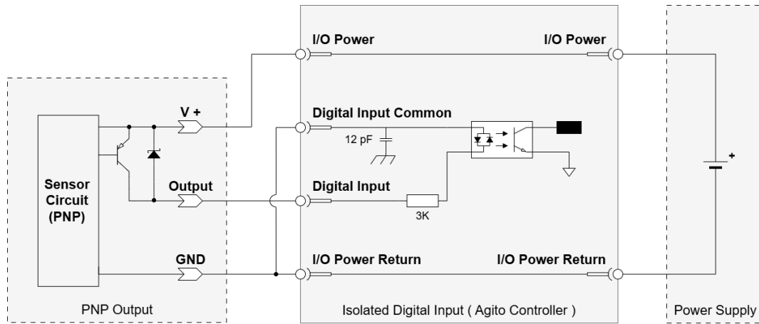
Figure 30. Digital Input with PNP Sensor
