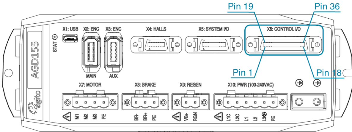
Figure 28. Control I/O Connector
