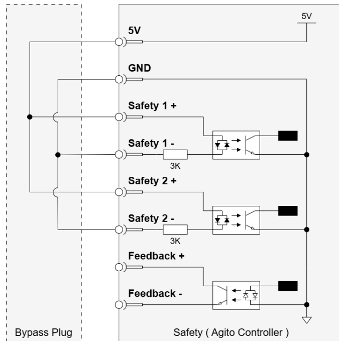
Figure 13. Safety Bypass
