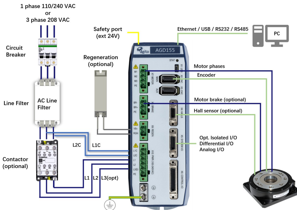
Figure 3. System Connection and Wiring (AGD155-AF)
