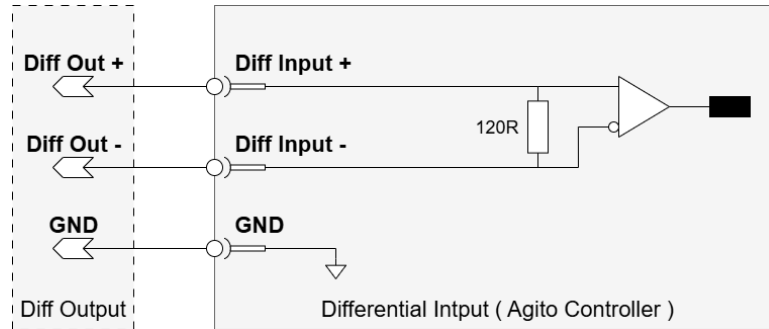
Figure 34. Differential Input
