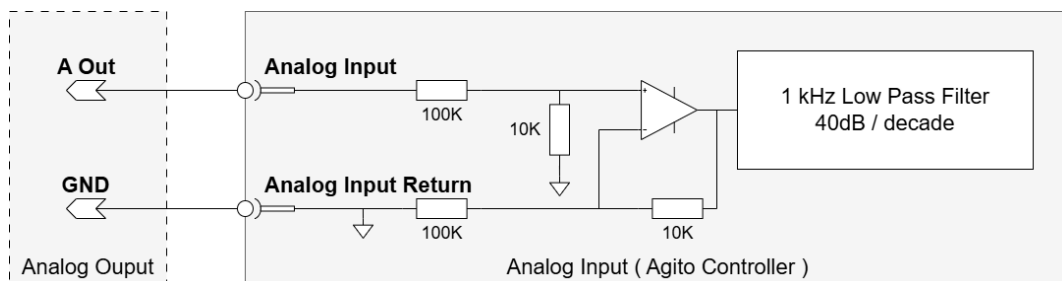
Figure 37. Analog Input
