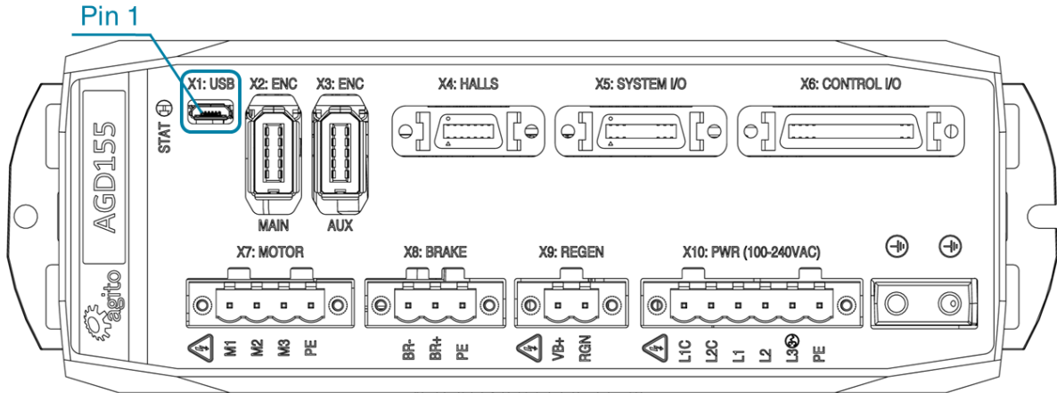
Figure 22. USB Connector
