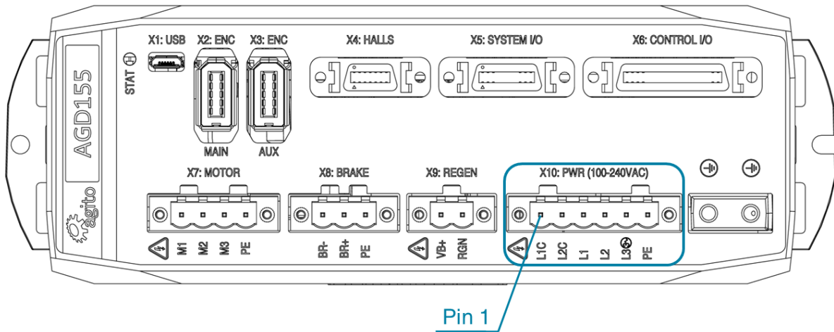
Figure 9. Power Connector
