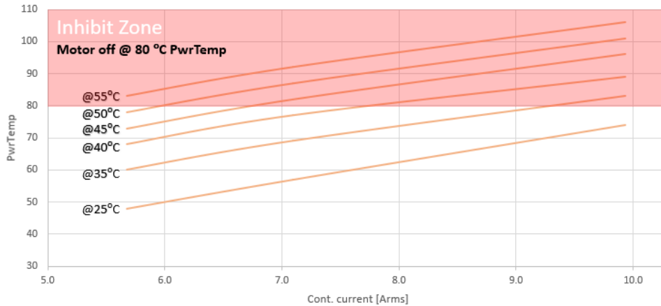
Figure 7. Current/Temperature
