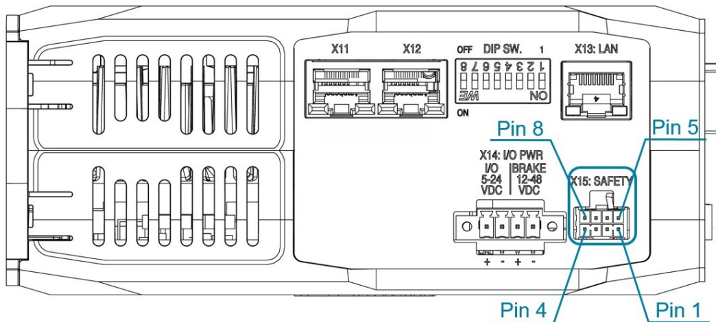
Figure 12. Safety Connector
