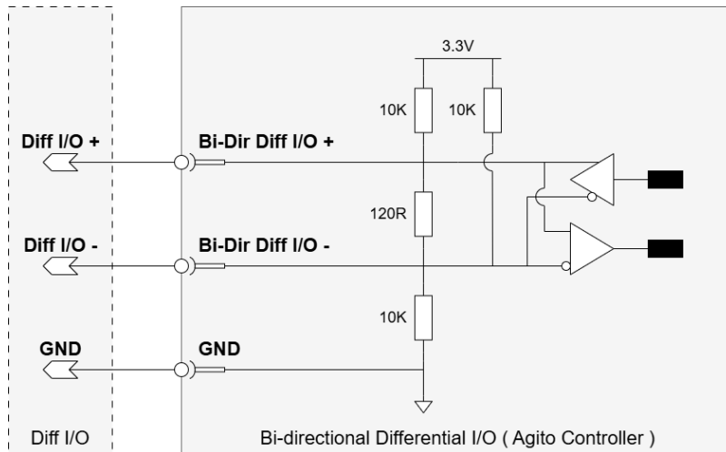
Figure 36. Bi-Directional Differential I/O
