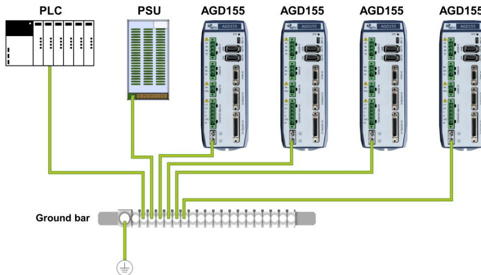
Figure 8. System Grounding
