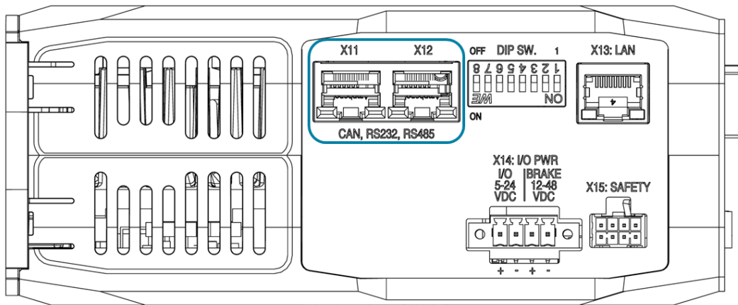
Figure 21. Serial Communication Connectors (AGD155-AF)
