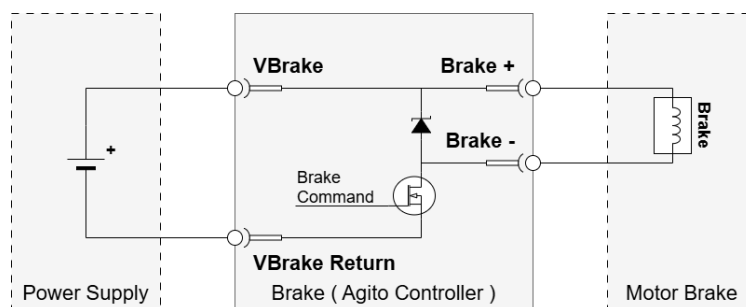
Figure 16. Brake
