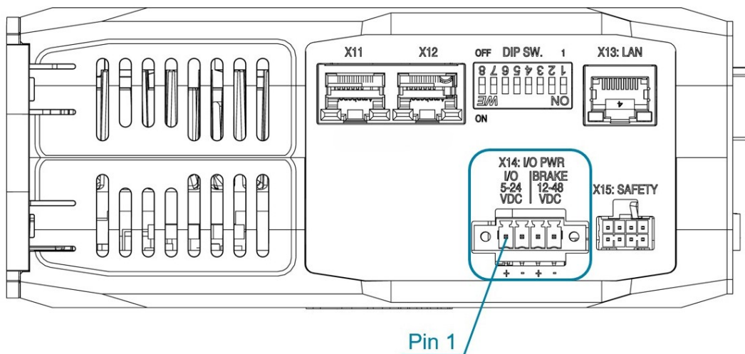
Figure 10. I/O and Brake Power Connector
