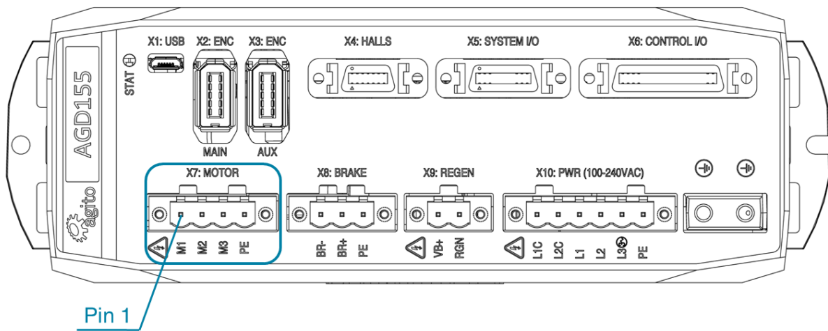
Figure 11. Motor Connector
