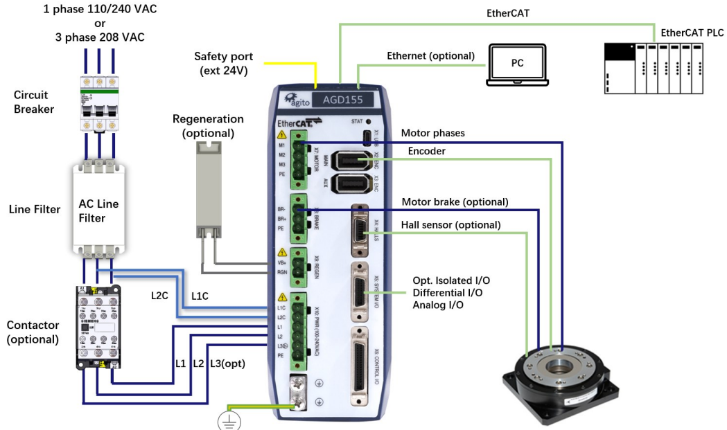
Figure 2. System Connection and Wiring (AGD155-EC)
