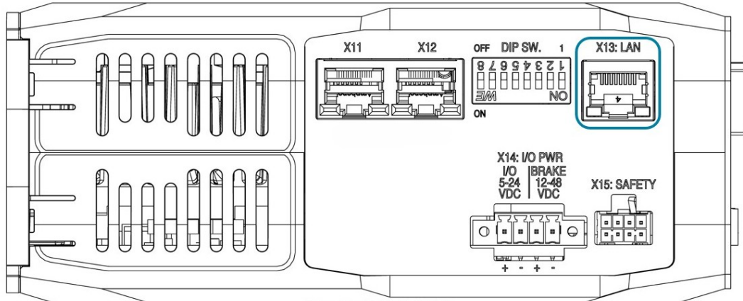
Figure 19. Ethernet Connector
