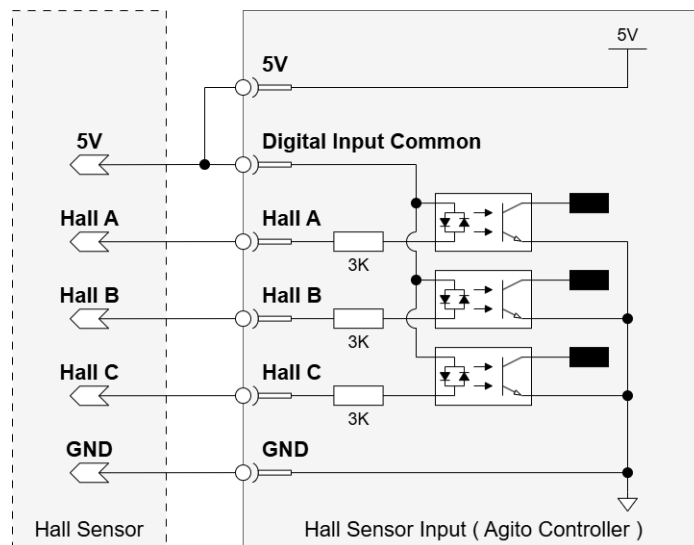
Figure 26. Hall Sensor
