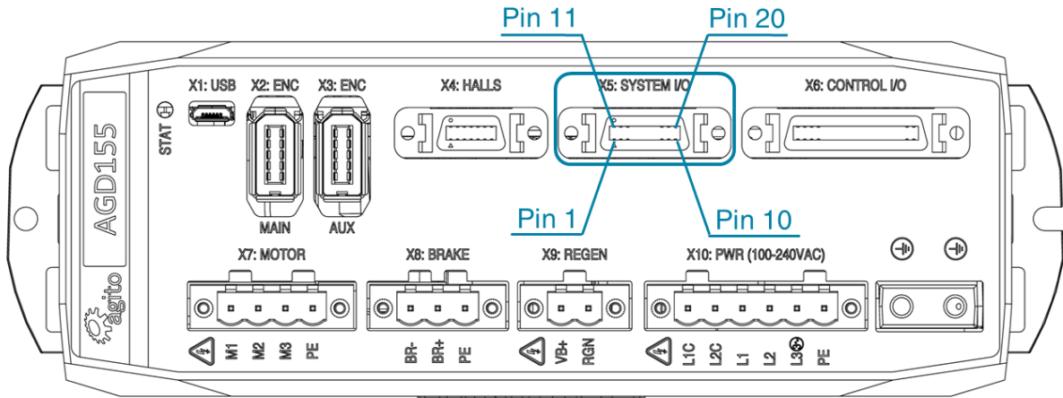
Figure 27. System I/O Connector
