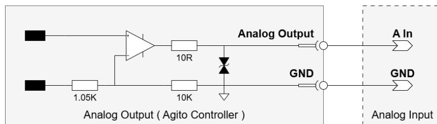
Figure 38. Analog Output
