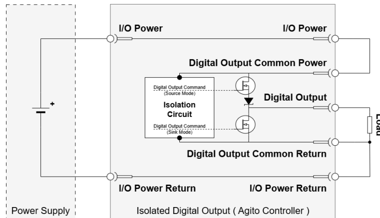
Figure 33. Digital Output (Source Mode)
