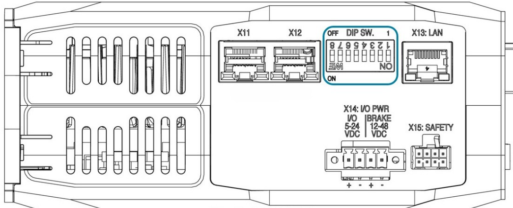
Figure 18. DIP Switches
