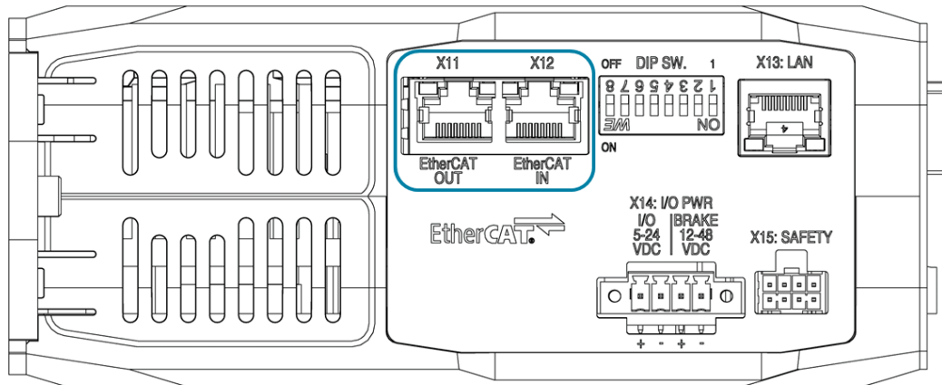
Figure 20. EtherCAT Connectors (AGD155-EC)
