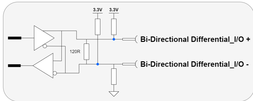
Figure 33. Bi-Directional Differential I/O
