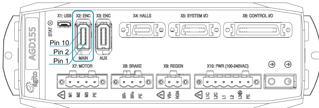
Figure 22. Main Encoder Connector
