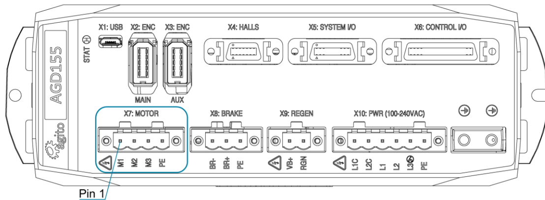
Figure 11. Motor Connector
