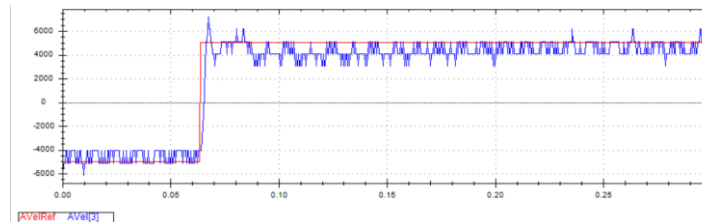
Figure 58. Typical Velocity Loop Performance
