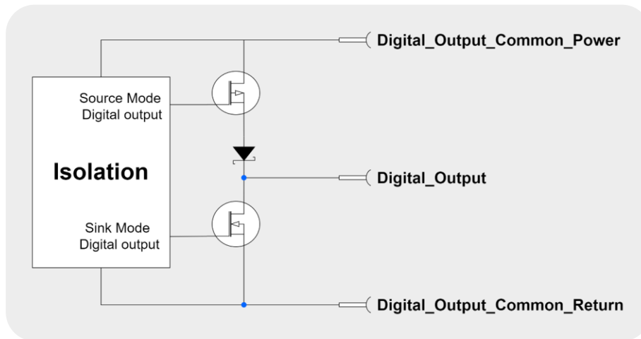
Figure 30. Digital Output 1 to 2, and 3 to 6 (2 isolated groups)
