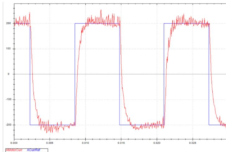
Figure 50 Typical Current Loop Performance
