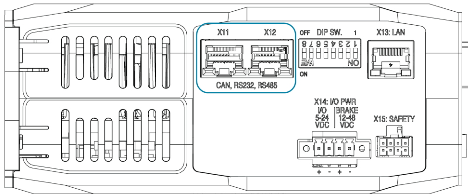
Figure 20: EtherCAT Connectors – AGD155-AF
