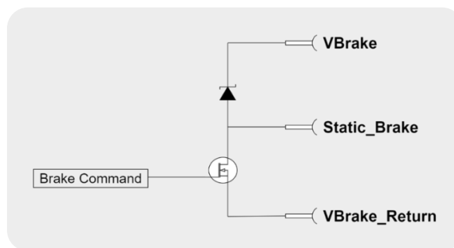
Figure 15. Static brake
