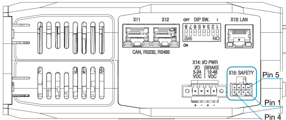
Figure 12. Safety Connector
