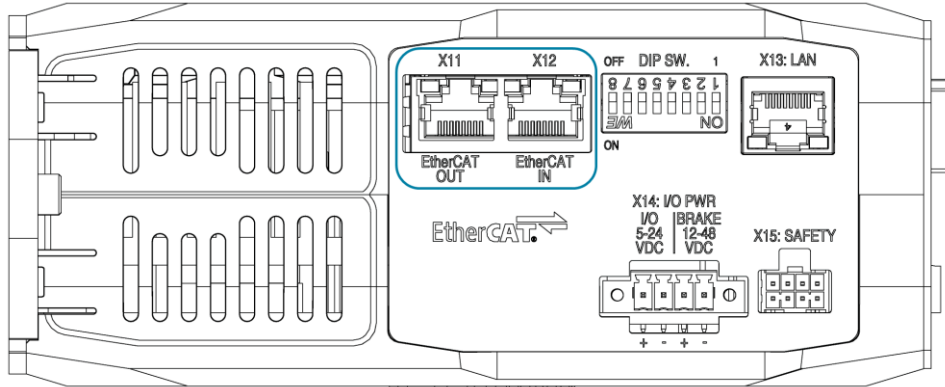
Figure 19: Serial Communication Connectors – AGD155-EC
