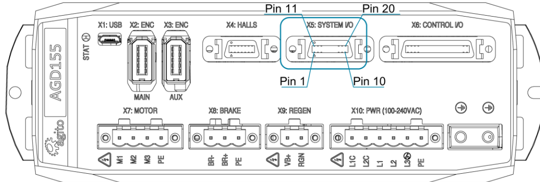
Figure 26. System I/O Connector
