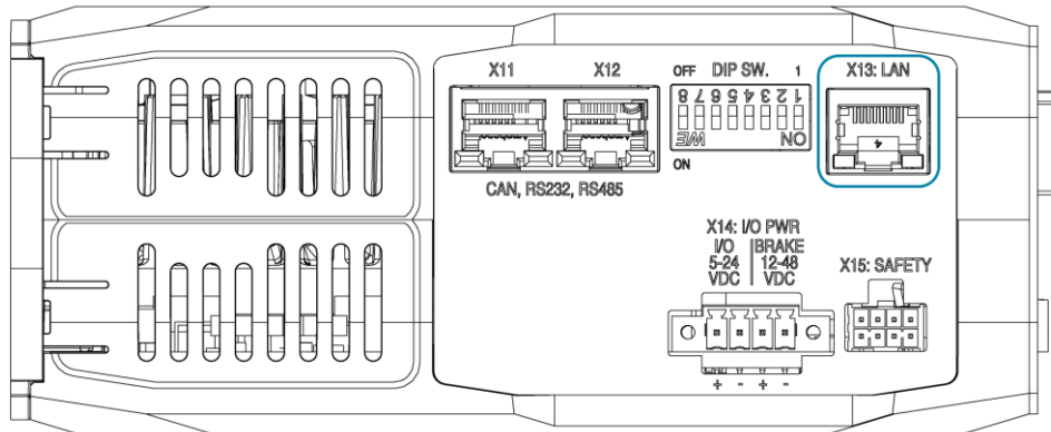
Figure 18: Ethernet Connector
