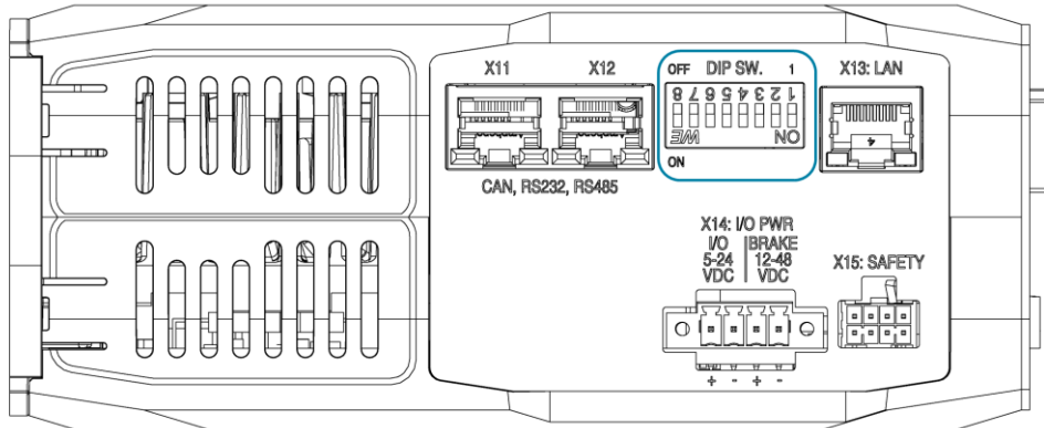
Figure 17 DIP Switches
