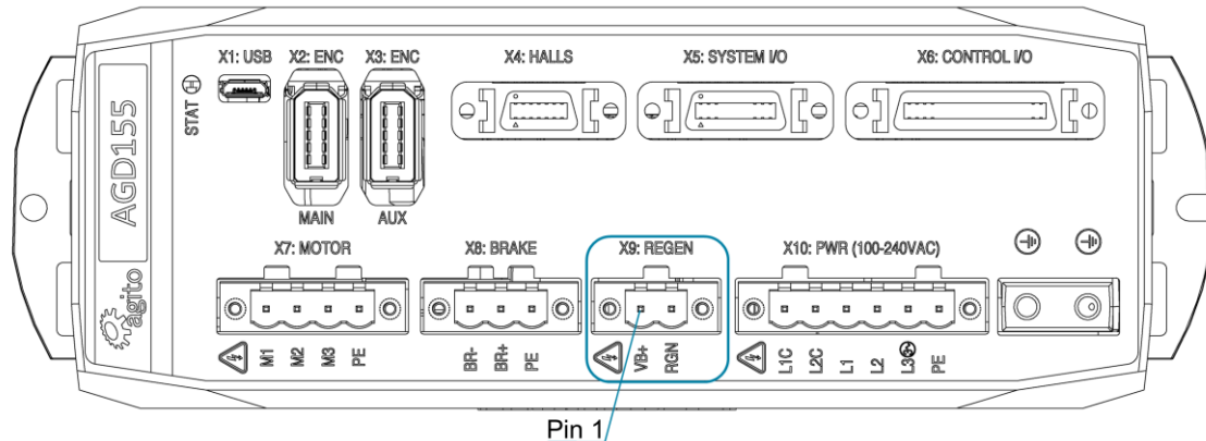
Figure 16. Regeneration Connector
