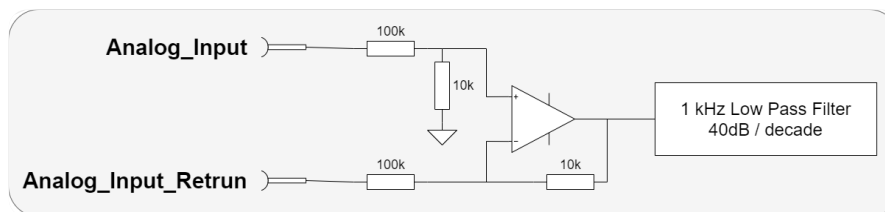
Figure 34. Analog Inputs 1 to 2
