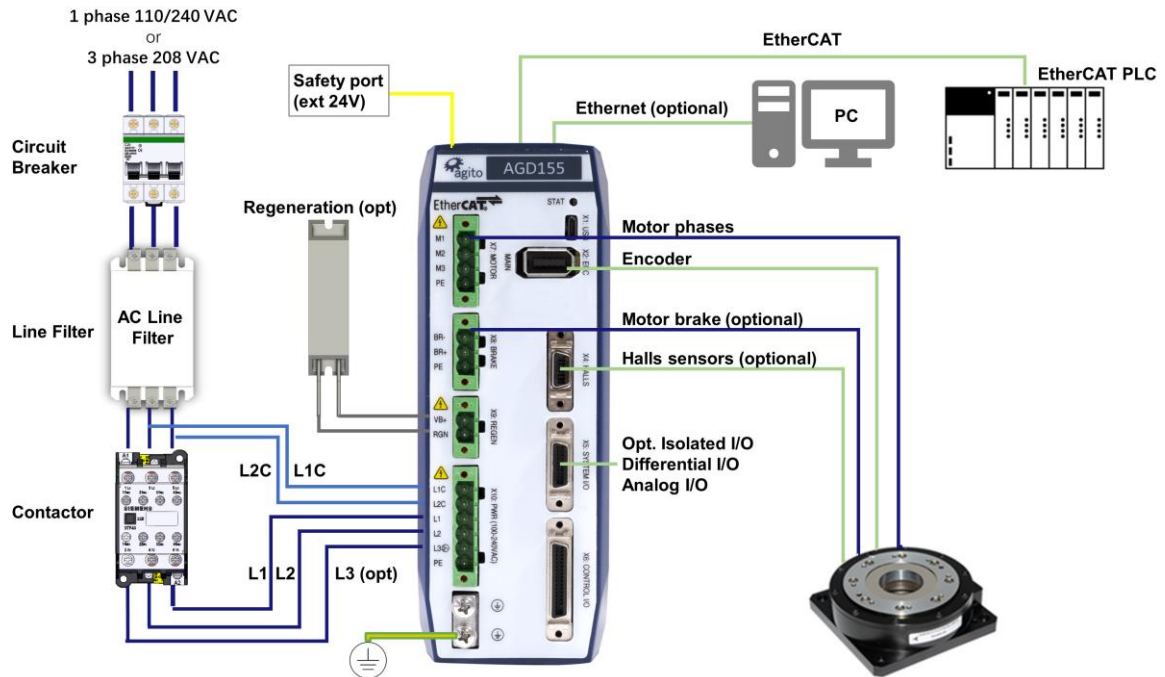
Figure 2. System connections and wiring – AGD155-EC
