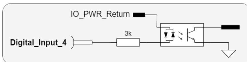
Figure 29. Digital Input 4
