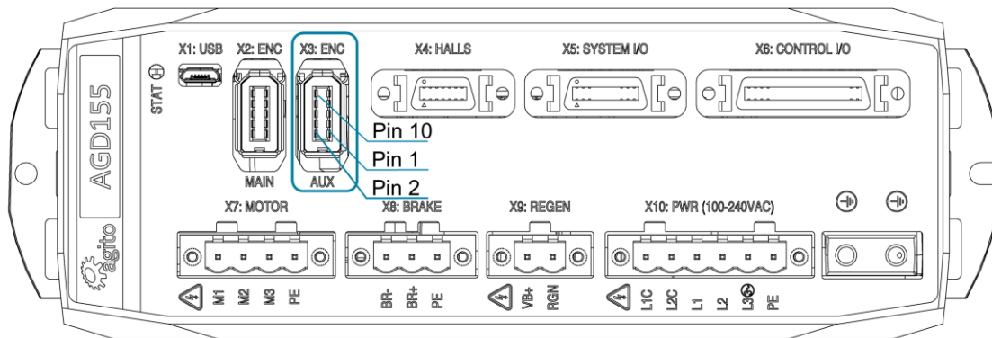
Figure 23 Aux Encoder Connector
