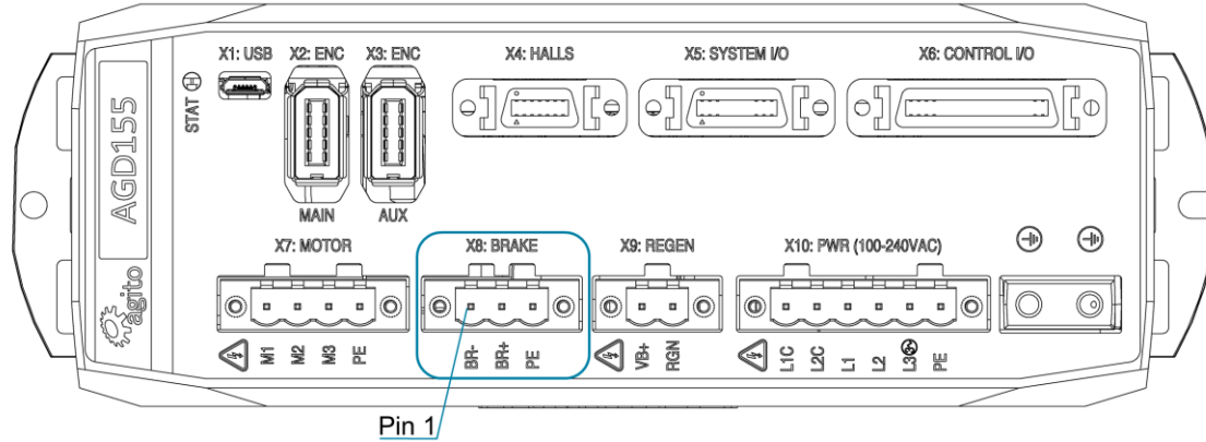
Figure 14. Brake Connector
