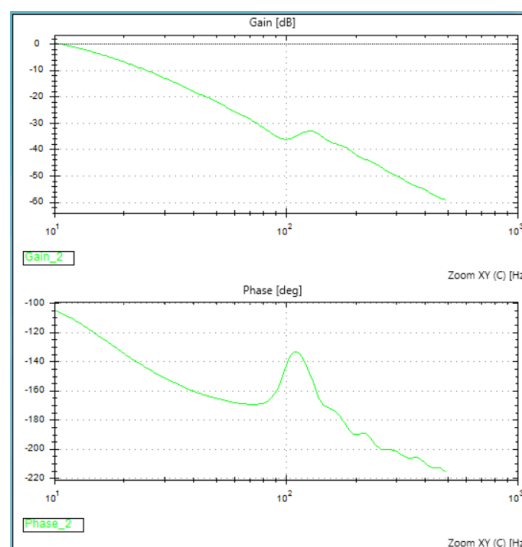
Figure 52. Typical Plant Transfer Function
