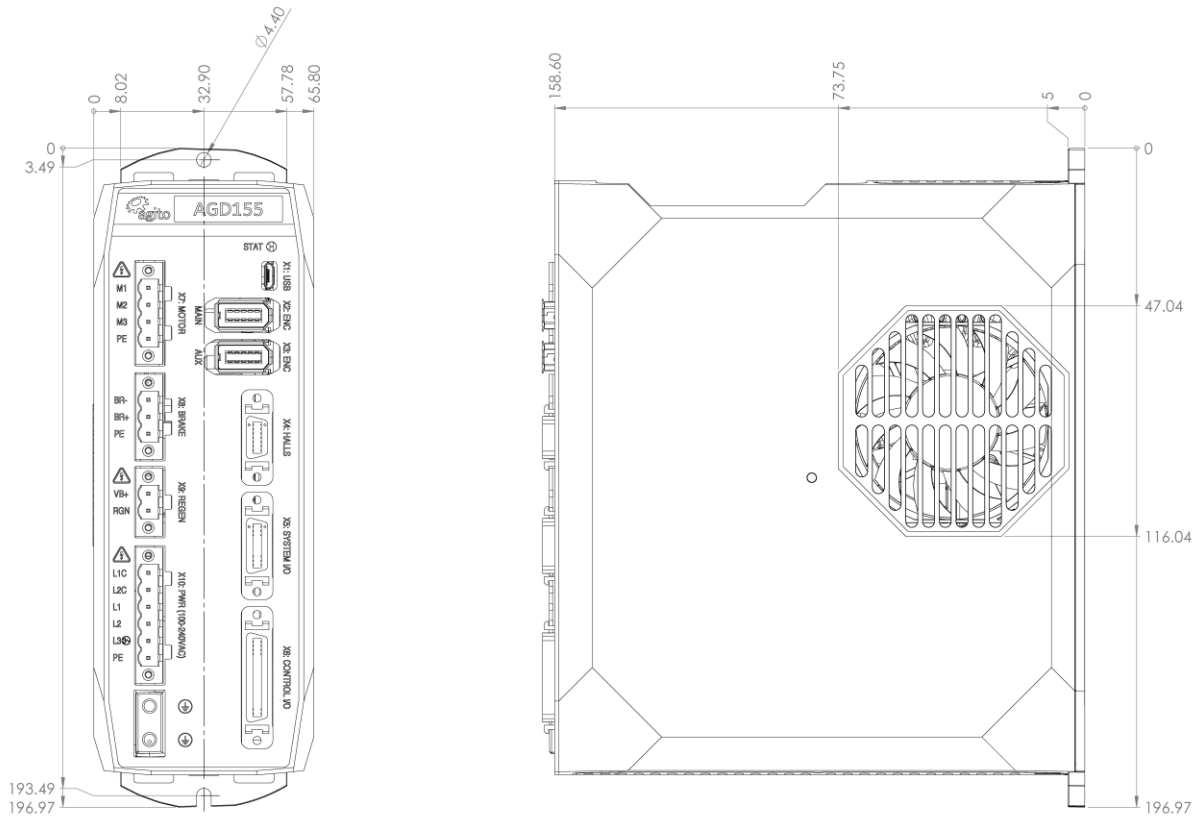
Figure 4. Product Dimensions (mm)
