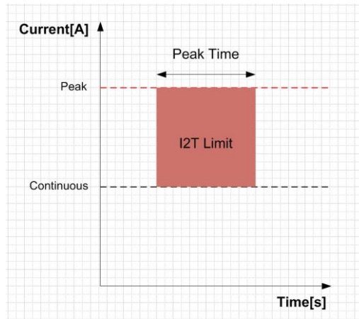
Figure 42. I^2T
