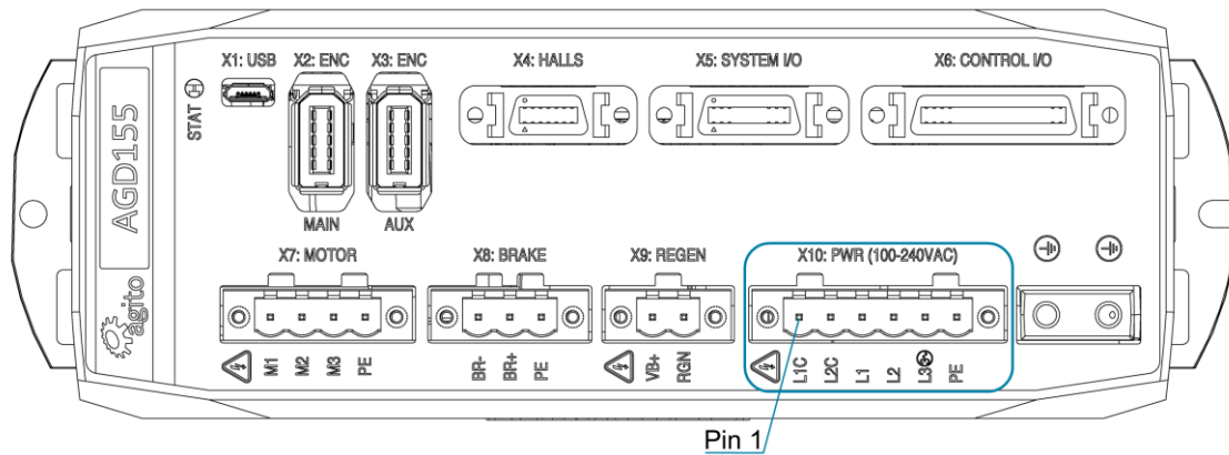
Figure 9. Power Connector
