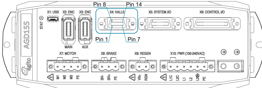
Figure 24. Hall Sensors Connector
