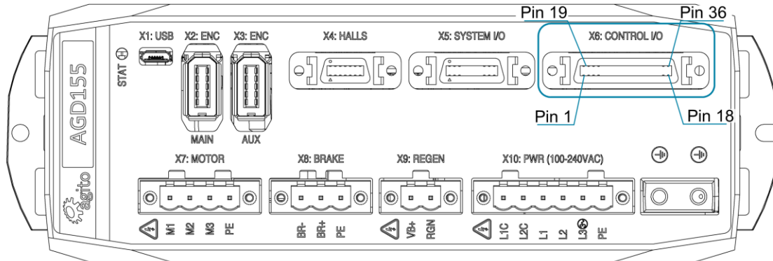
Figure 27: Control I/O Connector
