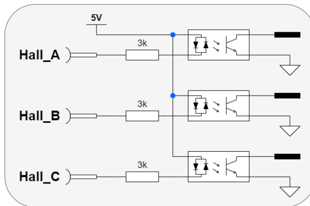
Figure 25. Hall sensors
