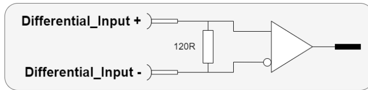
Figure 31. Differential Inputs 1 to 3
