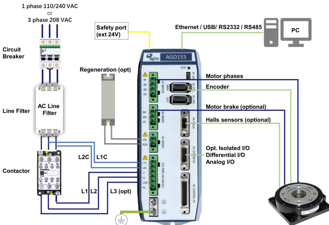
Figure 3. System connections and wiring – AGD155-AF
