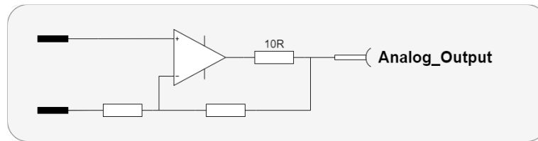
Figure 35. Analog Outputs 1 to 2
