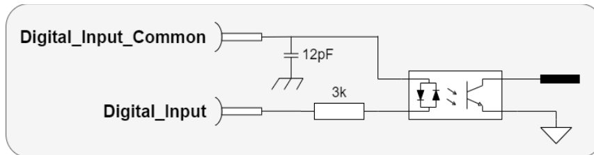
Figure 28. Digital Input 1 to 3, 5 to 9, and 12 to 16 (3 isolated groups)
