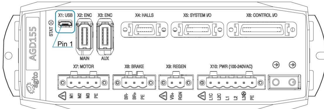
Figure 21: USB Connector
