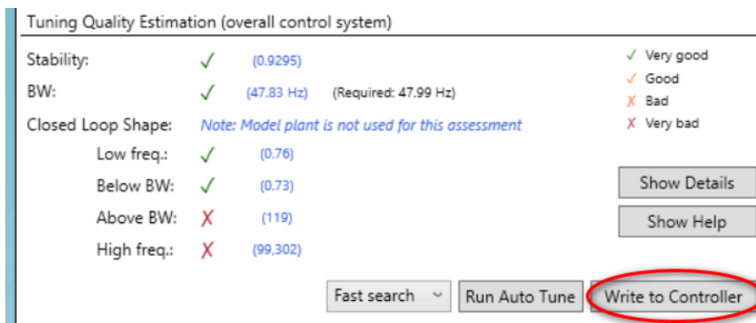
Figure 55. Download the parameters to the controller
